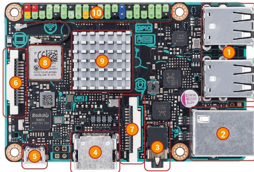
Figura 10: ASUS Tinker Board S
