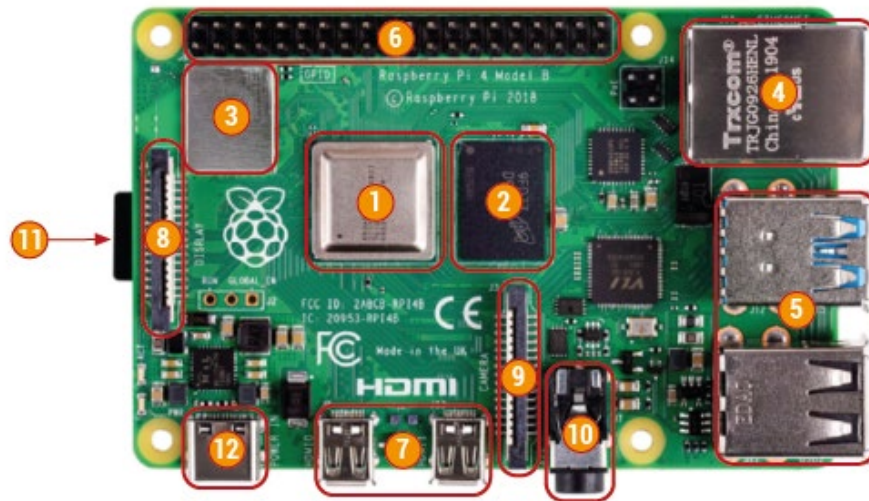
Figura 12: Raspberry Pi 4B
